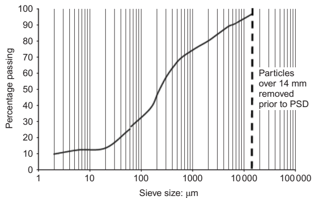
Fig. 2. Particle size distribution of rammed earth mix
