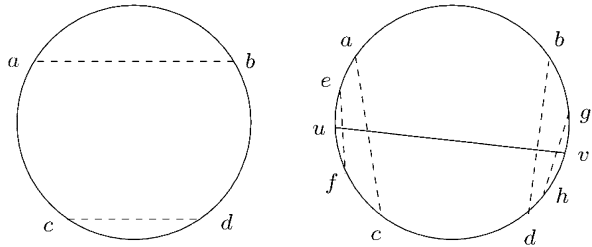
Fig. 9 On the left the original tree, and on the right the partition of the tree into two forests and a chord uv
