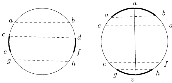
Fig. 8 On the left (resp. right), regions corresponding to Property T1 (resp. Property T2 ). Full lines correspond to real chords of C , dashed lines correspond to the limit of regions. Bold intervals correspond to intervals with no chord of C with both endpoints in the interval
