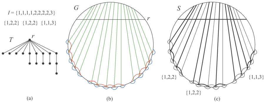
Fig. 7 Reduction in the proof of Theorem 4. (a) Instance I of 3-PARTITION, with n = 9 , m = 3 , and B = 5 , together with the associated tree T . (b) Circle graph G built from I . (c) The thick chords define a \{T\} -dominating set S in G
