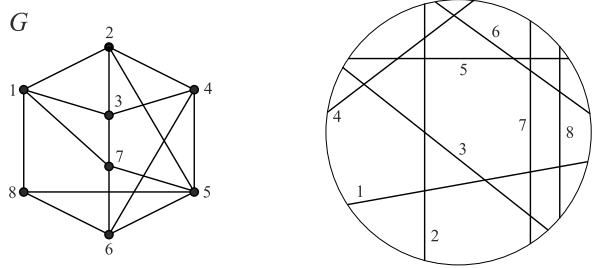
Fig. 1 A circle graph G on 8 vertices together with a circle representation of it
