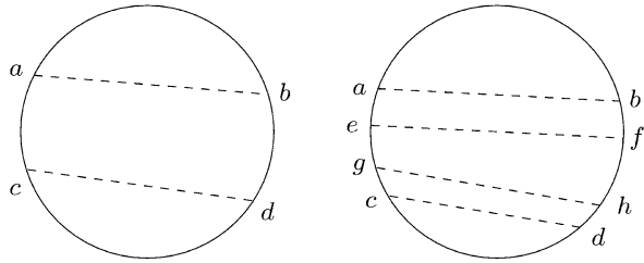
Fig. 10 On the left the original forest F , and on the right the partition of the forest into the two forests F_1 and F_2
