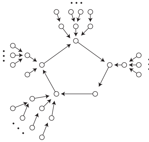
Figure 3: A representation of vertices firing
