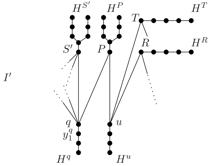
Figure 2: The graph G in Case 2.
