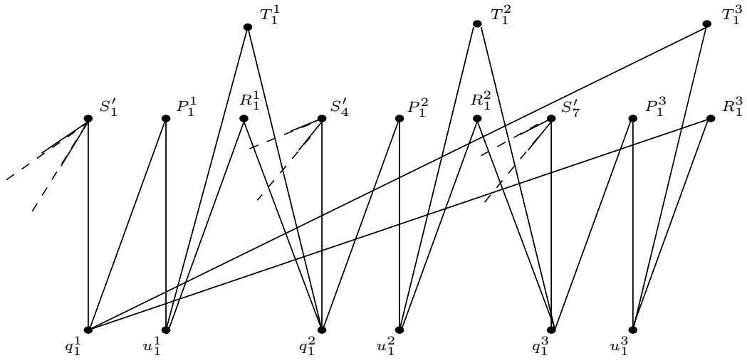
Figure 1: Part of the incidence graph of the triple of a hypergraph.
