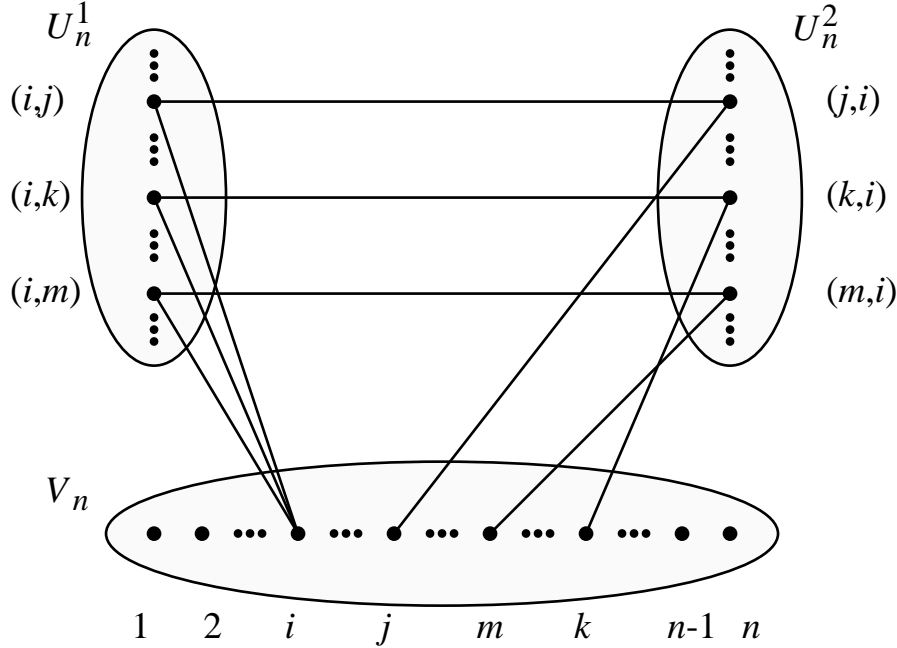
Figure 1. The graph H_n .
